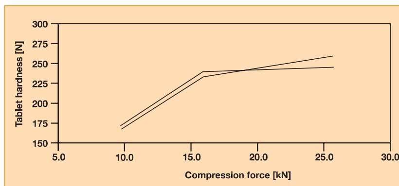
Fig. 3: Hardness-compression force profile of propranolol sustained release tablets containing 50% of Kollidon® SR (2 Lots, Formulation see chapter 6.2)
