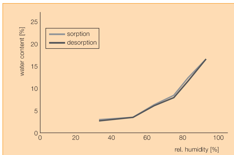
Fig. 2: Sorption isotherms of Kollidon® SR
