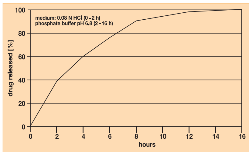
Fig. 8: Dissolution of theophylline sustained release tablets
