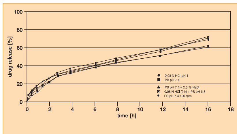
Fig. 5: Influence of the pH and the ionic strength of the dissolution medium on the release of caffeine tablets (Caffeine + Kollidon® SR 1+1)
