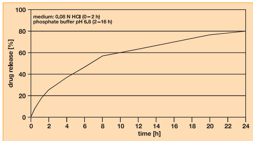
Fig. 7: Dissolution of Diclofenac sustained release tablets
